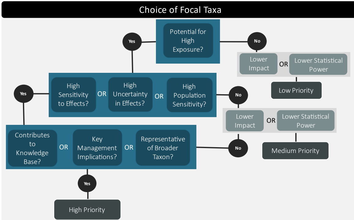
Figure 2. Decision tree to inform the choice of focal species for displacement, attraction, and macro- to meso-scale avoidance studies at offshore wind development sites. Definitions for the terms used in this figure are described below.
