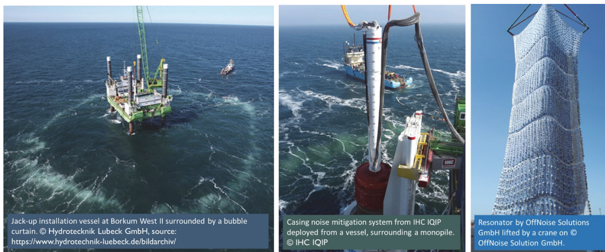
Figure 7. Examples of sound abatement systems including a bubble curtain (left), casing (middle), and resonator (right), figures adapted from Verfuss et al. 2019.
